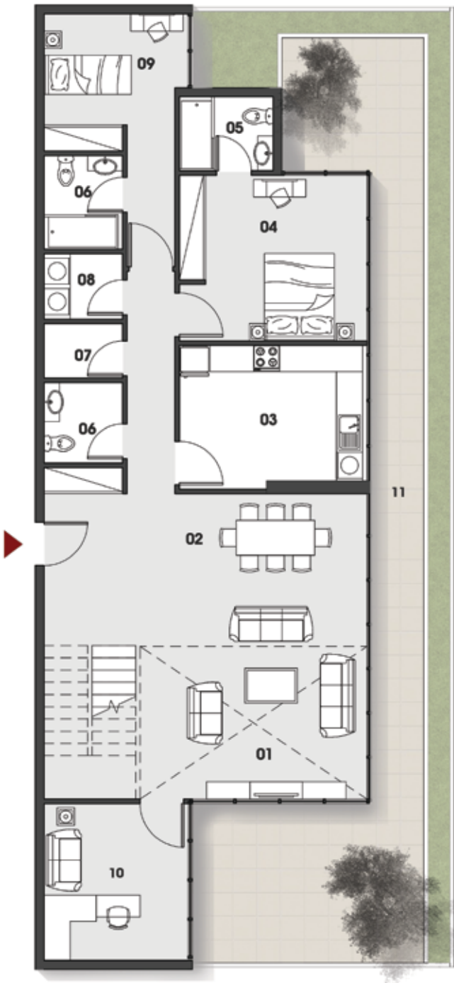
PENTHOUSE PLAN LOWER LEVEL
