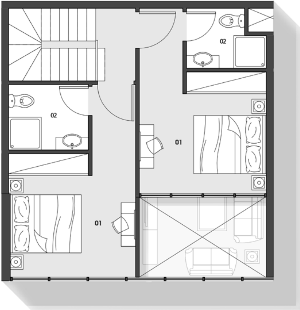
THREE BEDROOM LOFT PLAN UPPER LEVEL
